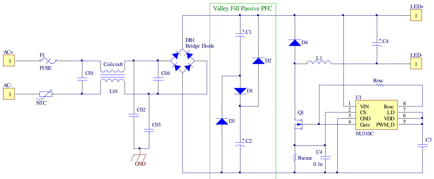
Figure 1: Typical Application Circuit with coilcraft and PFC
